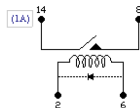
Wiring Diagram (Top View)
